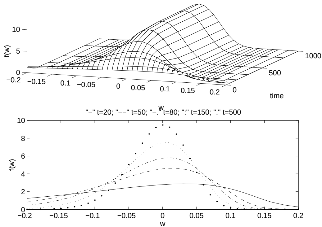
Figure 10.1: Density function for the estimates of the \alpha -parameter in the AR(1)-process in equation 10.38 for varying forgetting factor, \lambda , and varying estimation time.
