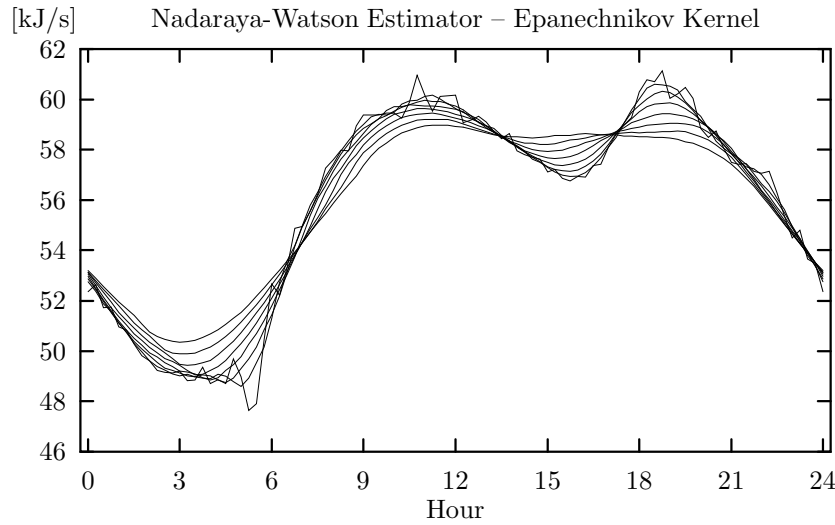
Figure 2.6: Smoothing of the diurnal power load curve using an Epanechnikov kernel and bandwidths 0.125, 0.625, . . . , 3.625.
