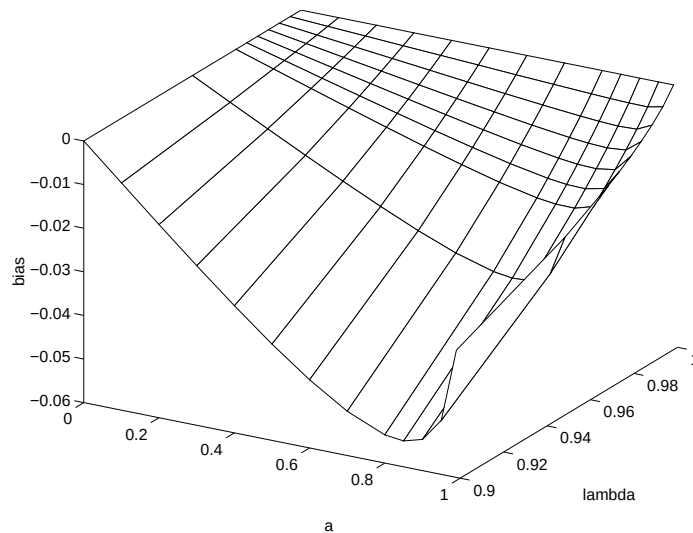
Figure 10.2: Exact asymptotic bias for the estimate of the \alpha -parameter in the AR(1)-process in equation 10.38 for varying forgetting factor, \lambda , and varying true parameter value.
