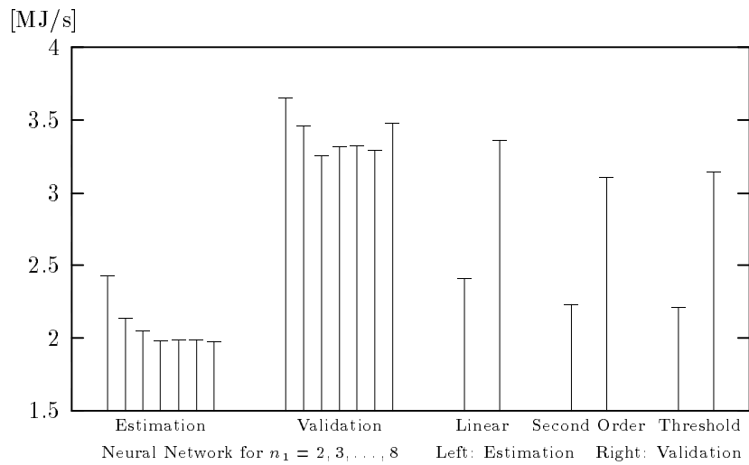
Figure 6.12: Bar diagram of \hat{\sigma}_e for the estimation set and \tilde{\sigma}_e for the validation set.
